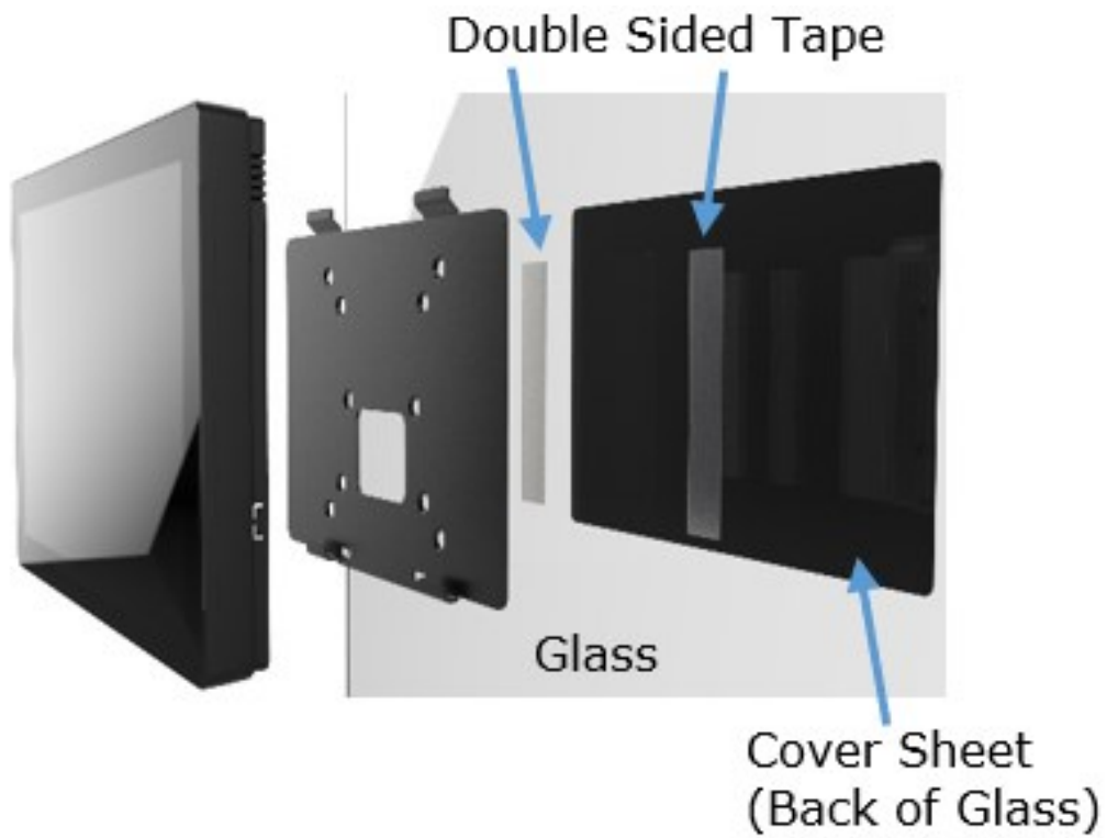
Figure 35 - Glass Mount
