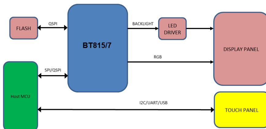
Figure 19 – Touch Host Mode Connection
