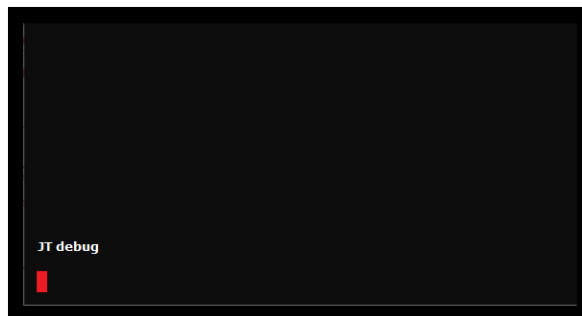
Figure 17 – Debugger Screen
