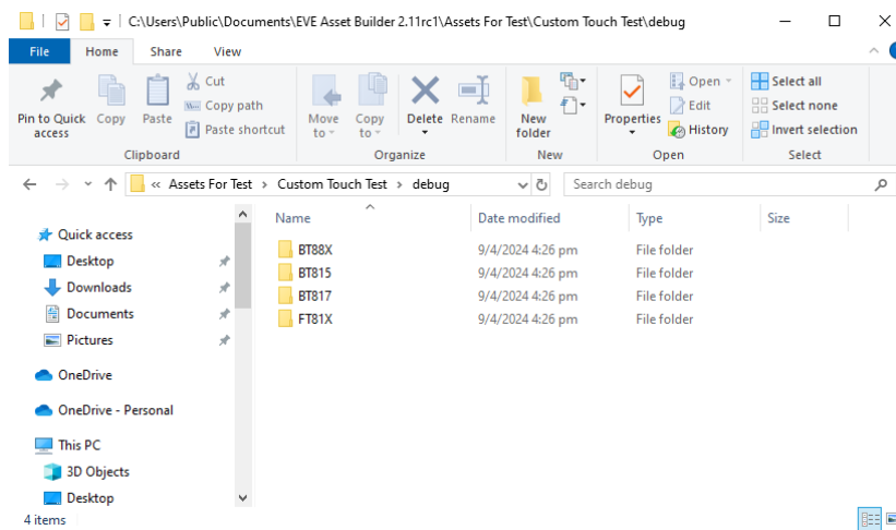
Figure 16 – debug folder
